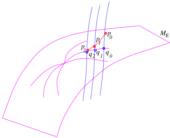
Fig. 2 An illustration of the “positive invariant” and “asymptotic phase” properties. Let p_0 be a point on the fiber W_\varepsilon^s(q_0) (vertical curve). Suppose the solution of (7) starting from q_0 \in M_\varepsilon evolves to q_1 \in M_\varepsilon at time \tau_1 , then the solution of (7) starting from p_0 will evolve to p_1 \in W_\varepsilon^s(q_1) at time \tau_1 . At time \tau_2 , they evolve to q_2, p_2 respectively. These two solutions are always on the same fiber. If we know that the one starting from q_0 converges to an equilibrium, then the one starting from p_0 also converges to an equilibrium
