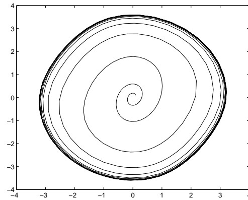
Fig. 9. Limit cycle in counterexample
