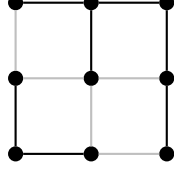
Figure 2: A forest in a 3 \times 3 grid.
