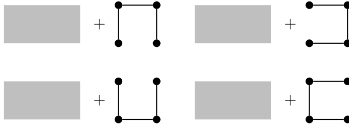
Figure 9: How we interpret 4T_{n-1} .
