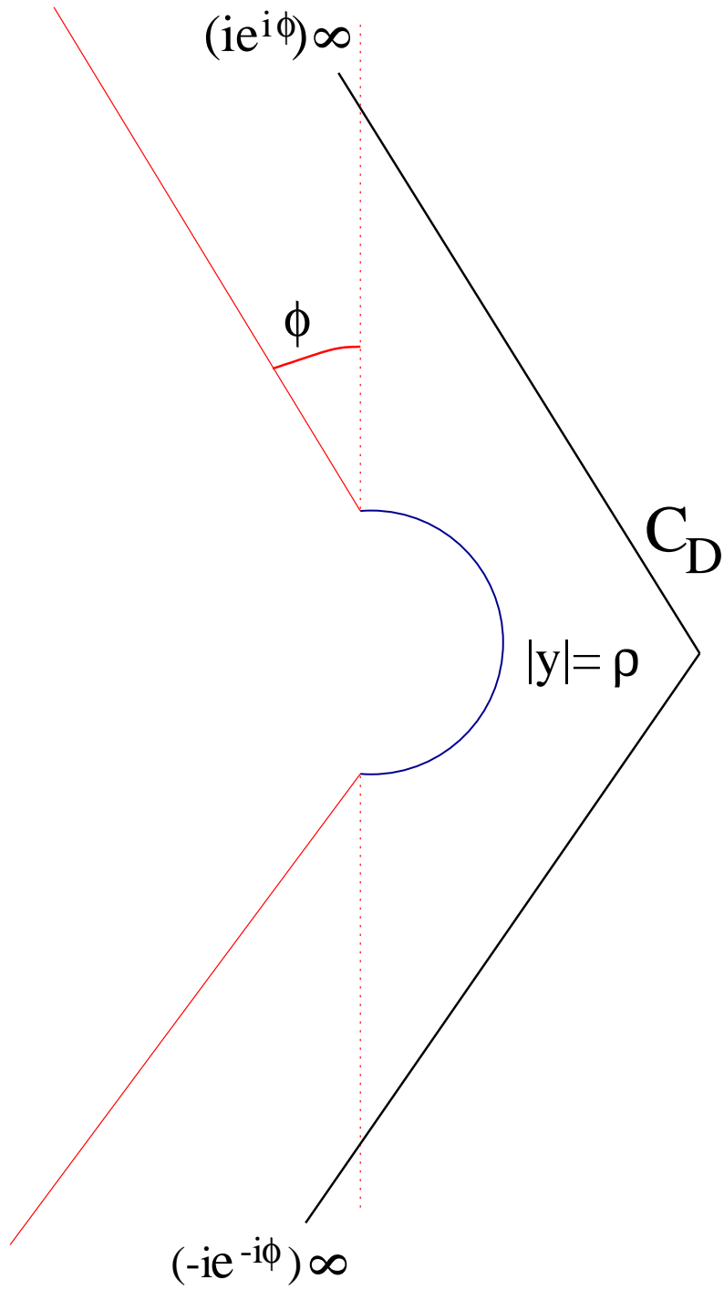
Fig. 1. Contour C_D in the (\mathbf{p})_i -plane.
